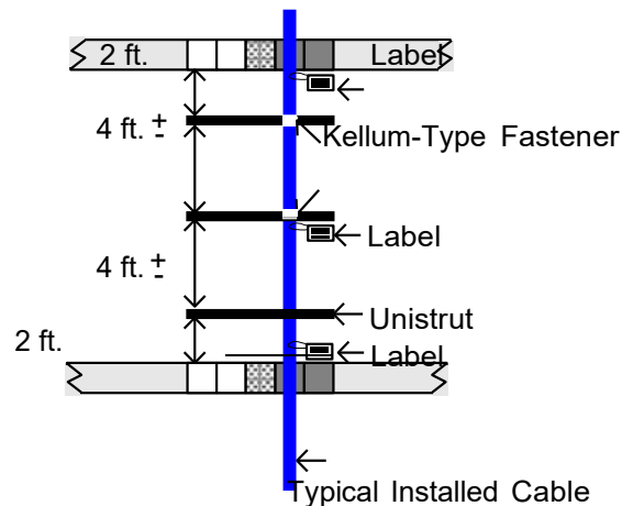
Cable support and label placement example
